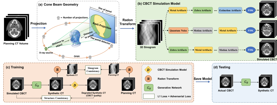
Fig. 2: Overview of the proposed framework. (a) A planning CT volume is first transformed into the 3D sinogram. (b) Simulated CBCT-specific artifacts are randomly applied to the sinogram, which are then transformed back to a CBCT-quality volume using the FDK algorithm. (c) The simulated CBCT is fed into the generative network trained with the proposed sinogram and structure consistency constraints. (d) During testing, the network takes the actual CBCT as input and outputs a denoised synthetic CT image.
