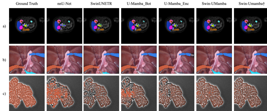
Fig. 2. Result visualization on a) AbdomenMRI, b) Endoscopy, and c) Microscopy.
