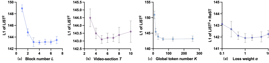
Fig. 3: Sensitivity analysis of our LiST 2 : (a) block number L , (b) section length T , and (c) global token number K , as well as (d) \mathcal{L}_{overlap} weight \alpha used in ReST
