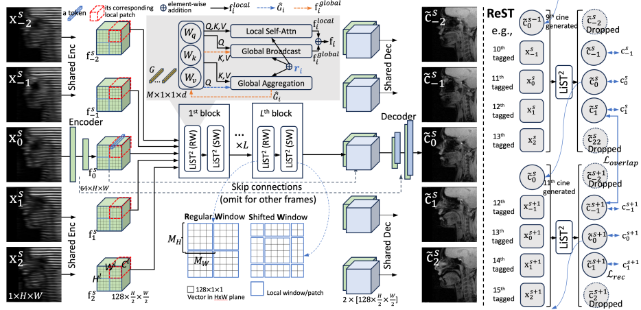
Fig. 1: Illustration of our video tagged-to-cine synthesis framework. Left: the UNet model with LiST 2 module. Right: ReST phase tuning with overlap loss.
