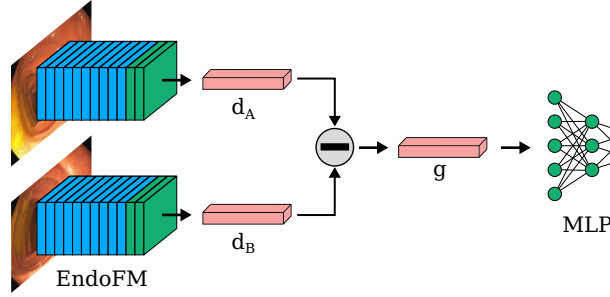
Fig. 2. Localization network \mathbb{L} . It obtains a sim score, deciding if two images come from the same place. The backbone green blocks and the MLP are fine-tuned.
