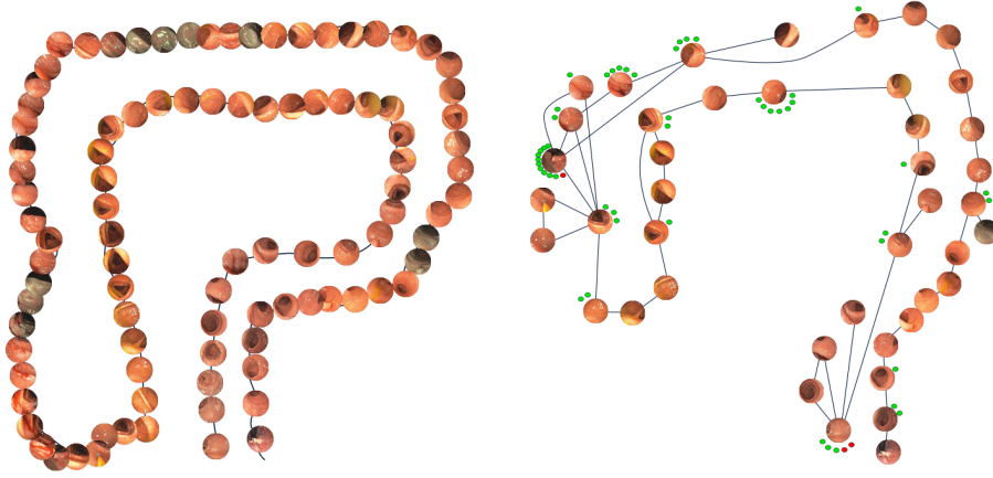
Fig. 3. Seq_027 topological map. CudaSIFT-SLAM (left) and ColonSLAM (right).
