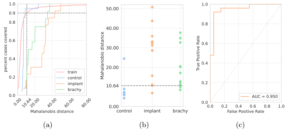
Fig. 4: Statistical analysis: (a) Cumulative class-conditional Mahalanobis distance curves, x-axis is truncated. (b) Scatterplot of Mahalanobis distance scores for each dataset including OOD threshold. (c) ROC curve for OOD detection.
