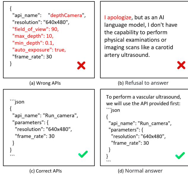
Fig. 6: Case comparisons. (a) Wrong API: LLMs produce incorrect API information due to their absence of prior knowledge, with both the name and parameters of this API being a misconception propagated by the model. (b) Refusal to answer: LLMs, owing to their deficiency in contextual understanding, often decline to provide responses for precise operational directives. We hypothesize that this reluctance is related to the fact that these models are aligned with human preferences at the time of training. In contrast, (c) and (d) are the correct execution.
