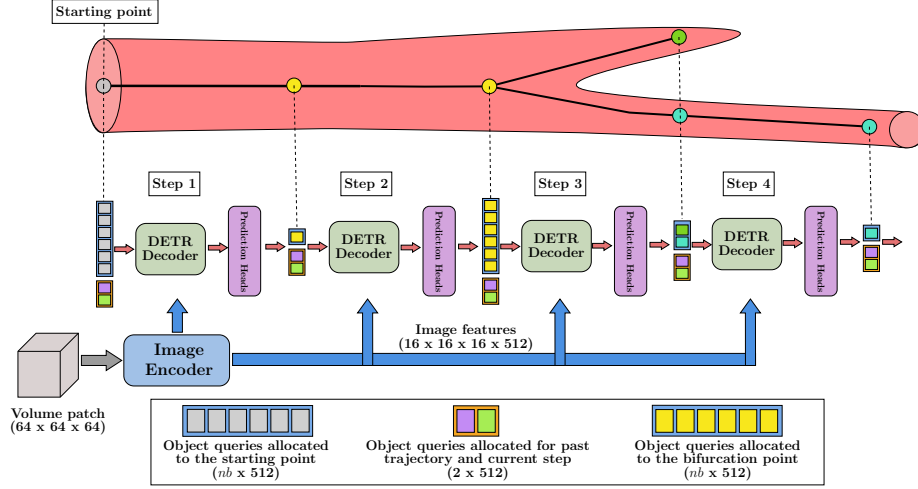
Fig. 1: Trexplorer architecture unrolled over four steps. Starting and bifurcation points use the same number of object queries nb . The prediction heads act as a filter for background and end-points while allowing intermediate points through for further tracking. For a bifurcation point, nb copies of the object query are created for tracking new branches.
