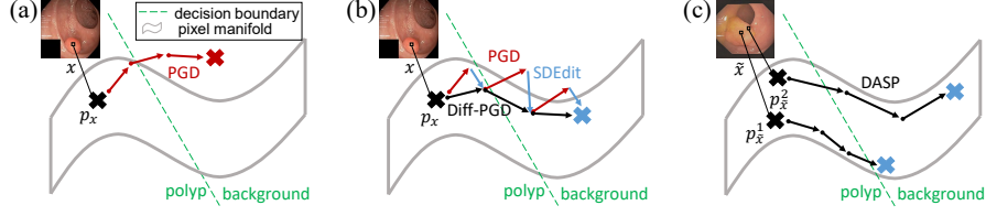
Fig. 1: (a) Adversarial attack using PGD. (b) PGD with SDEdit. (c) PGD with SDEdit considering per-pixel uncertainty.
