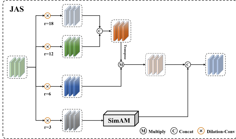
Fig. 2. The detail of the joint attention structure feature fusion module, Where r represents the step size of dilated convolution
