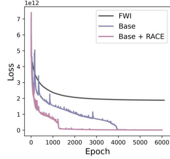
Fig. 5. Loss curve comparisons on numerical phantom.
